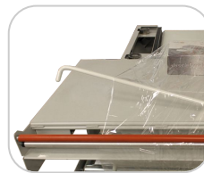
Film tracking roller and film separator for easy packaging loading
